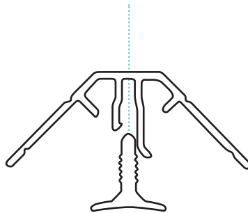
2-part Internal Corner Profile 90°
