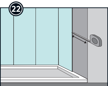
Measure last panel on return wall, cut to size, apply Fibro Seal on cut surfaces and attach to wall with glue
