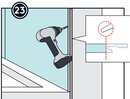
Countersink and attach with screws into stud with maximum ¼ inch from the edge. The screw will be hidden with L-profile
