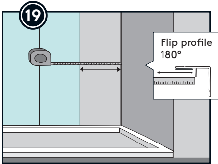
Flip the corner profile, measure and cut panel. Dry fit before applying glue and Fibro Seal.
