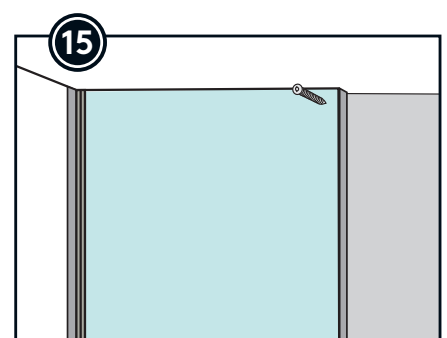
Countersink and attach with screw 1/4 inch from the top and into the stud. The screw will be hidden with L-profile
