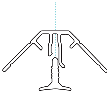
2-part Internal Corner Profile 90°
