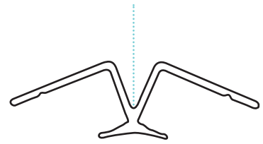
Internal Corner Profile 135°
