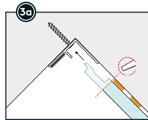
Attach the corner profile with screws. Slide the first panel into the corner profile.
