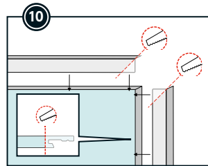
Measure and cut finishing profile/L-profile. Dryfit before applying it with Fibo Seal onto the panel. Remove excess sealant with Fibo Clean, Fibo Sealing Tools and finish with Fibo Wipes.
