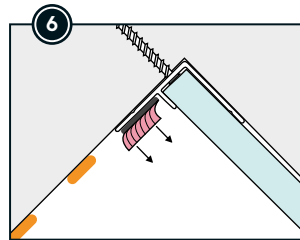
Remove tape film from the corner profile.
