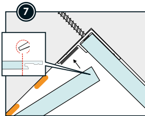
Adjust the last panel before clicking it into place.
