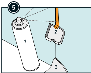
1. Spray with Fibo Clean 2. Remove with Fibo Sealing Tool 3. Finish with Fibo Wipes
