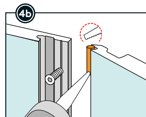
Place an installation screw in the screw lip on the right hand side of the panel. The screws will replace glue/Fibo Seal on the backwall. Apply Fibo Seal in the sealing lip on the left hand side of the next panel.
