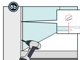
Clean cut the last panel. Attach a screw on the edge before the finishing L-profile is installed.
