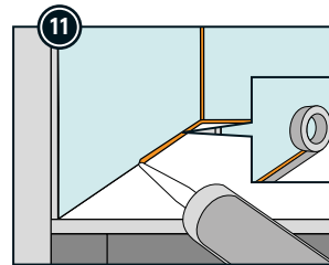
Place a masking tape on the worktop before sealing. Use Fibo Seal to hide transition between Kitchen Board and worktop. Make sure to remove all excess sealant with Fibo Clean, Fibo Sealing Tools and Fibo Wipes.
